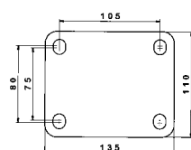
Ø 100/73-100/105
