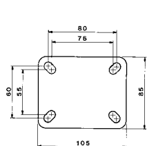
Ø 100/40
