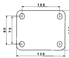
Ø 125/60-300/60
