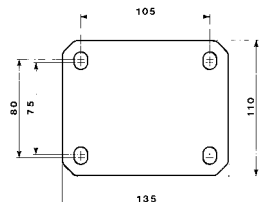
Ø 160/60-200/60
